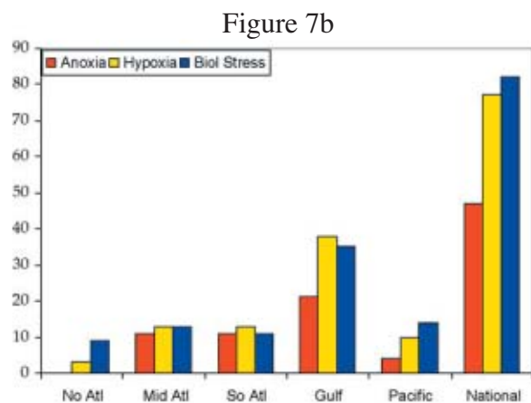
Figures 7a-c. The spatial area (a), the number of estuaries (b), and probable months of occurrence (c) of anoxia (0 mg/L dissolved oxygen [DO]), hypoxia (> 0 but ≤ 2 mg/L DO) and biologically stressful concentrations of dissolved oxygen (>2 but ≤ 5 mg/L DO) in United States estuaries. Figures are not meant to show cross-regional differences, but rather to highlight qualitative intra-regional differences (e.g., There are no reported incidences of anoxia within the Northern Atlantic Region). (Adapted from Bricker et al. 1999).
