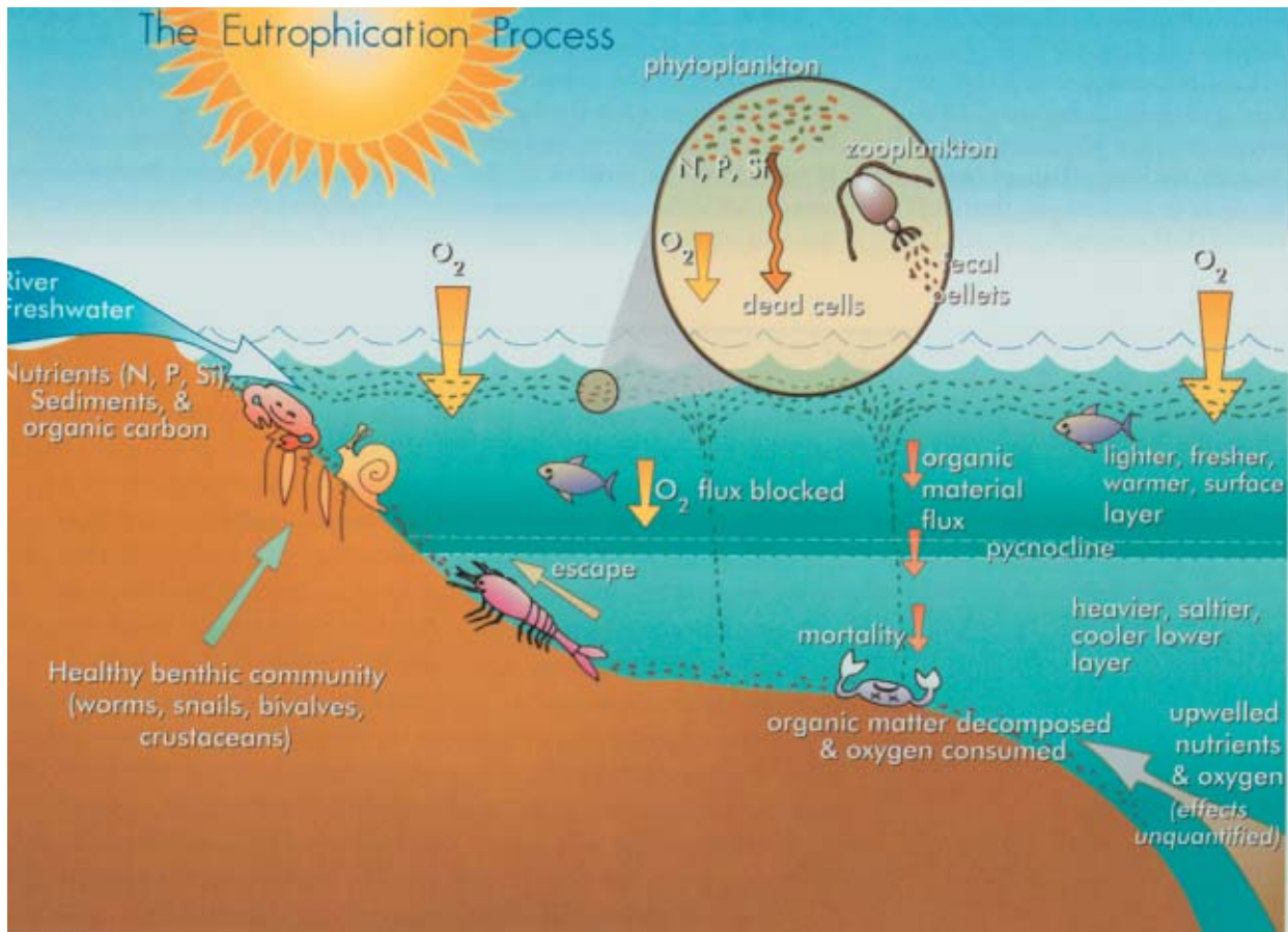
Figure 1. The Eutrophication Process. Eutrophication occurs when organic matter increases in an ecosystem through nutrient stimulated algal growth or through inputs of organic matter from other sources. (Adapted from CENR 2000a)
