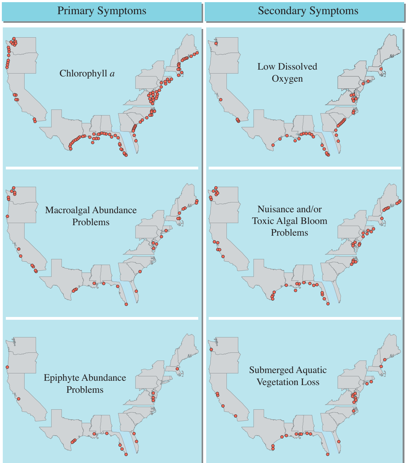
Figure 6. Expression of Eutrophic Symptoms. The following maps depict estuaries with moderate to high levels of expression of the symptoms listed in Box 1, indicating areas of possible concern. These symptoms are not necessarily related in whole to human-related nutrient inputs; natural causes and other human disturbances may also play a role to varying degrees in the expression of symptoms. (Adapted from Bricker et al. 1999)
